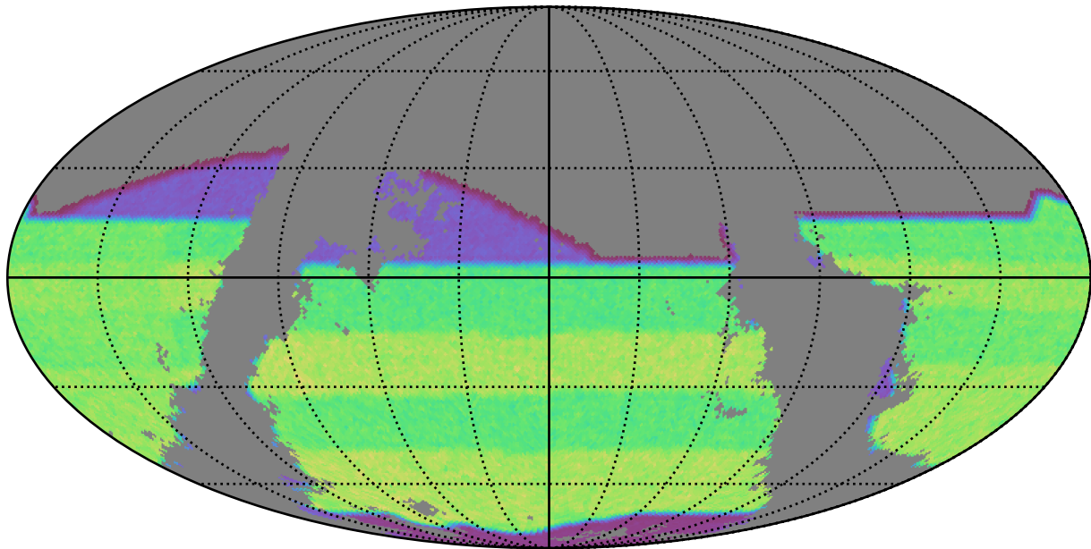
ddf_half_v3.4_10yrs gri band non-DD: riz_exposure_time_year9
