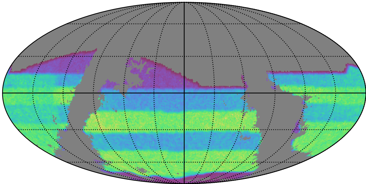
ddf_half_v3.4_10yrs gri band non-DD: gri_exposure_time_year3
