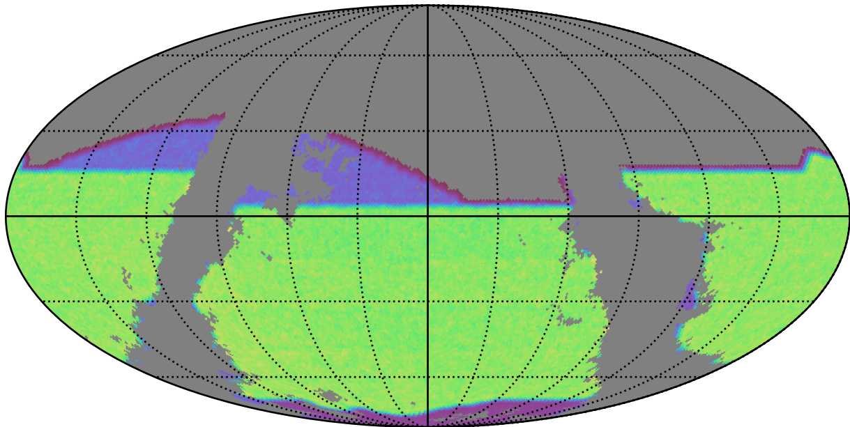
ddf_half_v3.4_10yrs gri band non-DD: gri_exposure_time_year10
