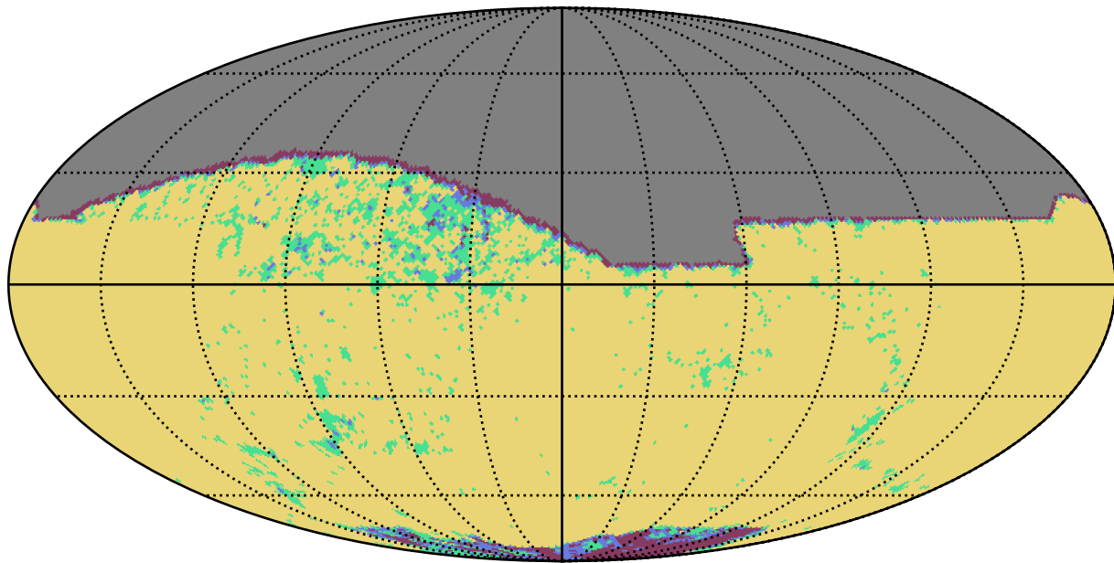
ddf_half_v3.4_10yrs z band: YearCoverage night
