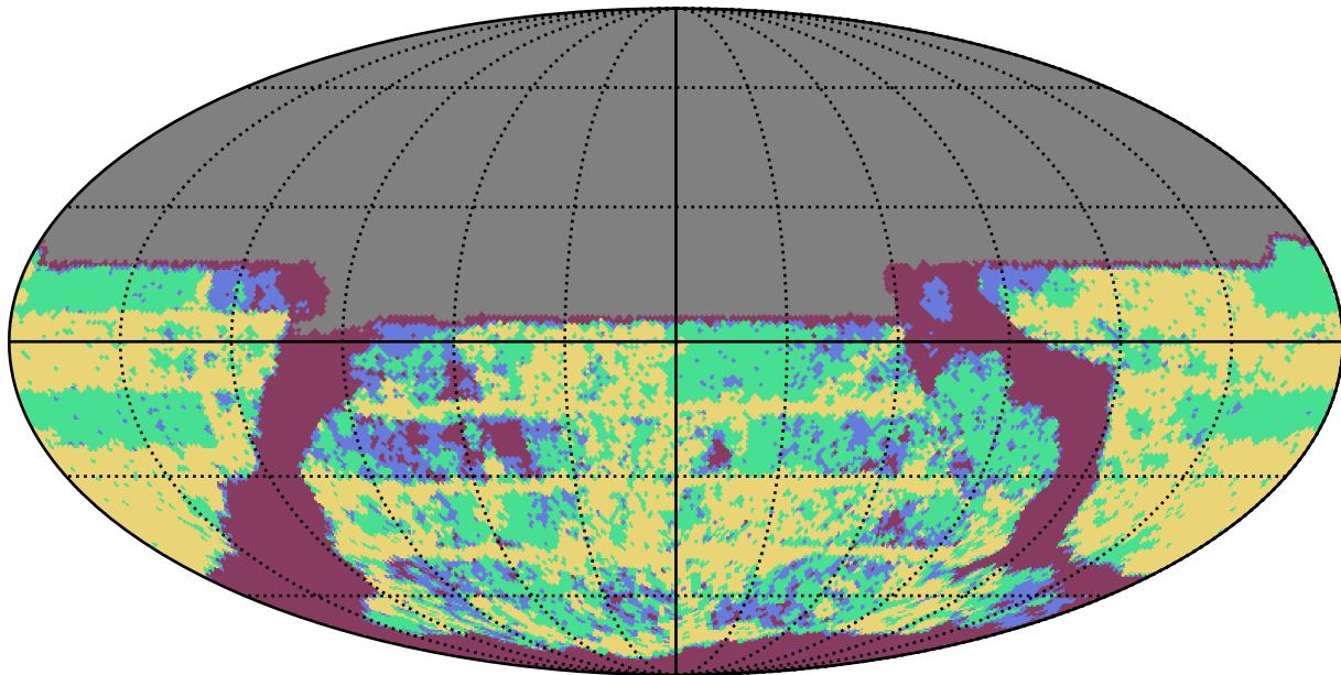
ddf_half_v3.4_10yrs u band: YearCoverage night
