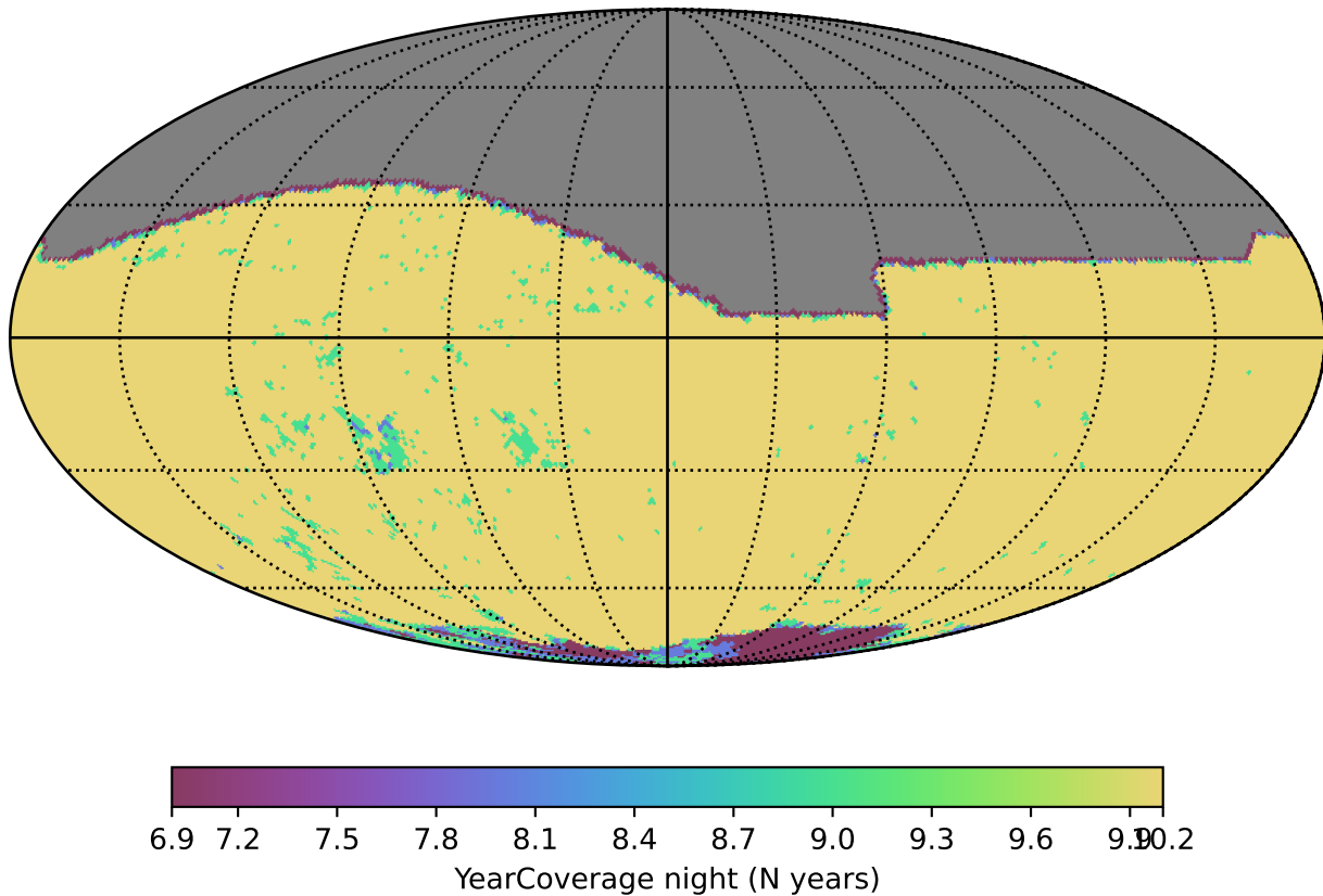
ddf_half_v3.4_10yrs r band: YearCoverage night
