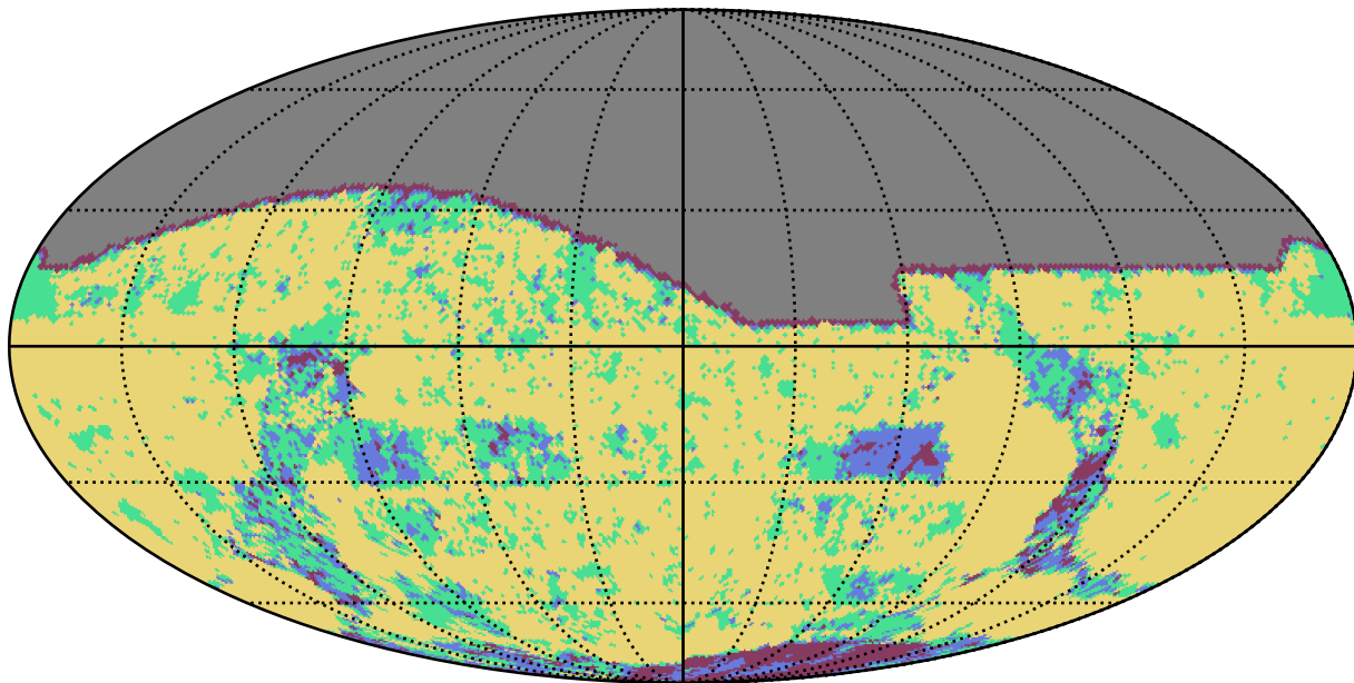
ddf_half_v3.4_10yrs g band: YearCoverage night
