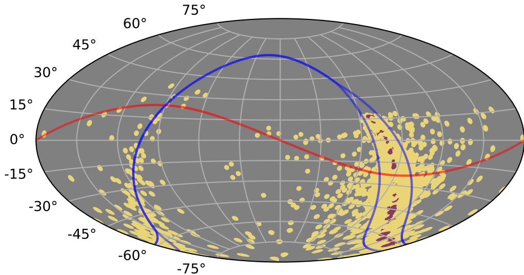
ddf_half_v3.4_10yrs : XRBPopMetric_possible_to_detect
