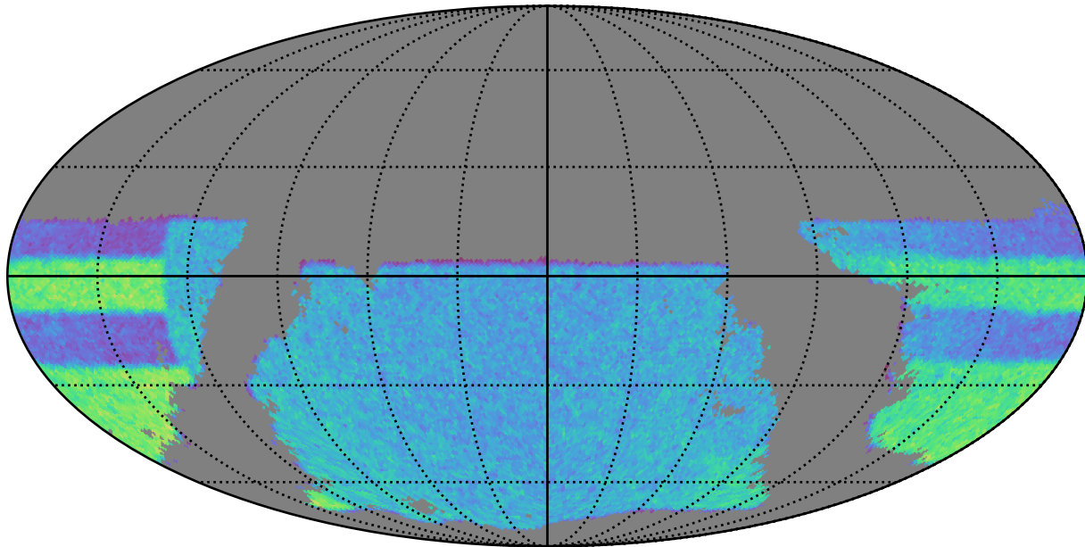
ddf_half_v3.4_10yrs gri band non-DD: WeakLensingNvisits_riz_year2
