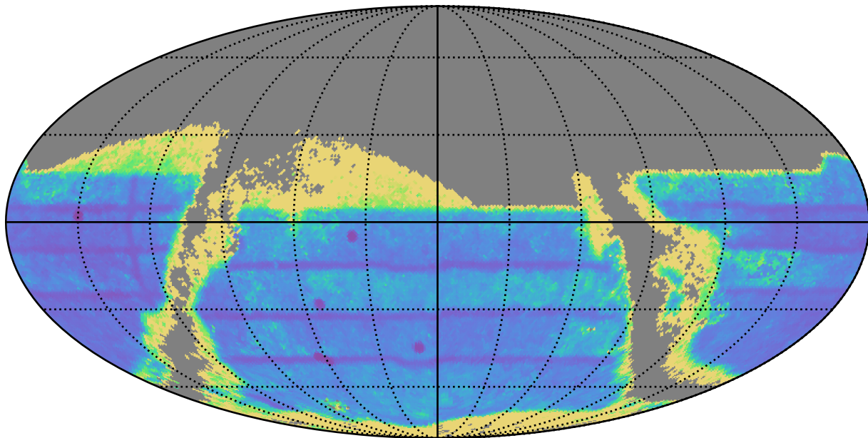
ddf_half_v3.4_10yrs : TDC_precision
