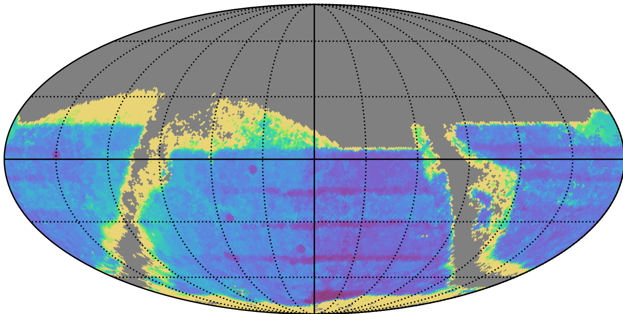
ddf_half_v3.4_10yrs : TDC_accuracy
