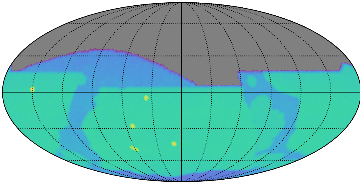
ddf_half_v3.4_10yrs z: SurfaceBrightLimit
