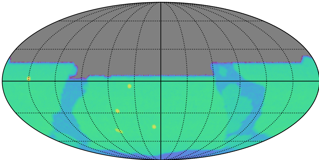
ddf_half_v3.4_10yrs y: SurfaceBrightLimit
