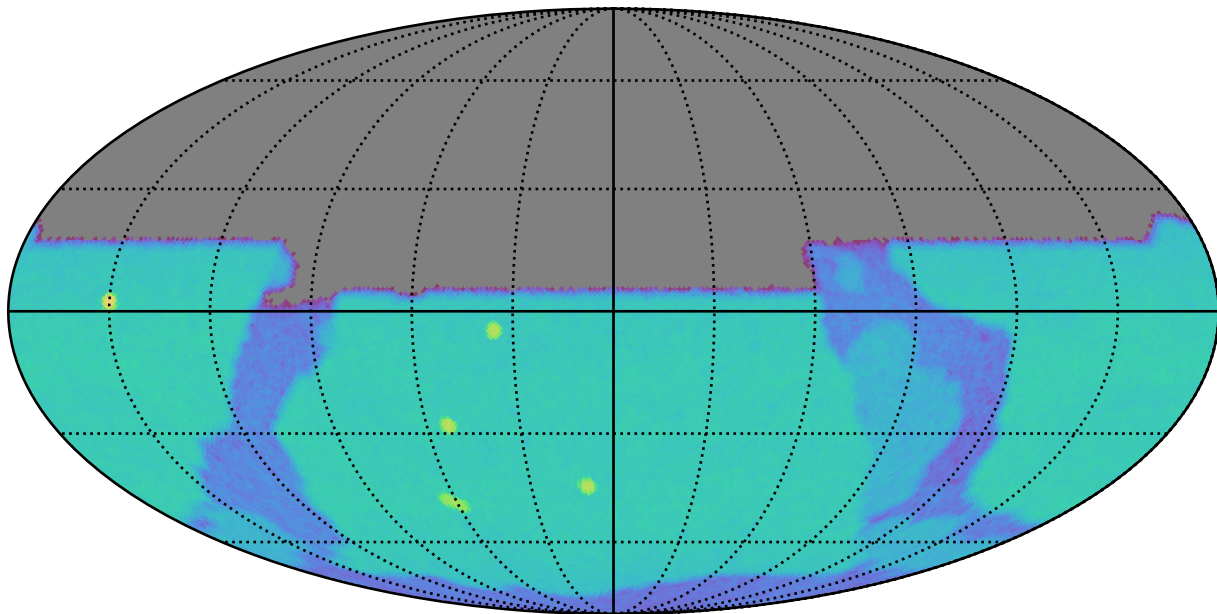
ddf_half_v3.4_10yrs u: SurfaceBrightLimit
