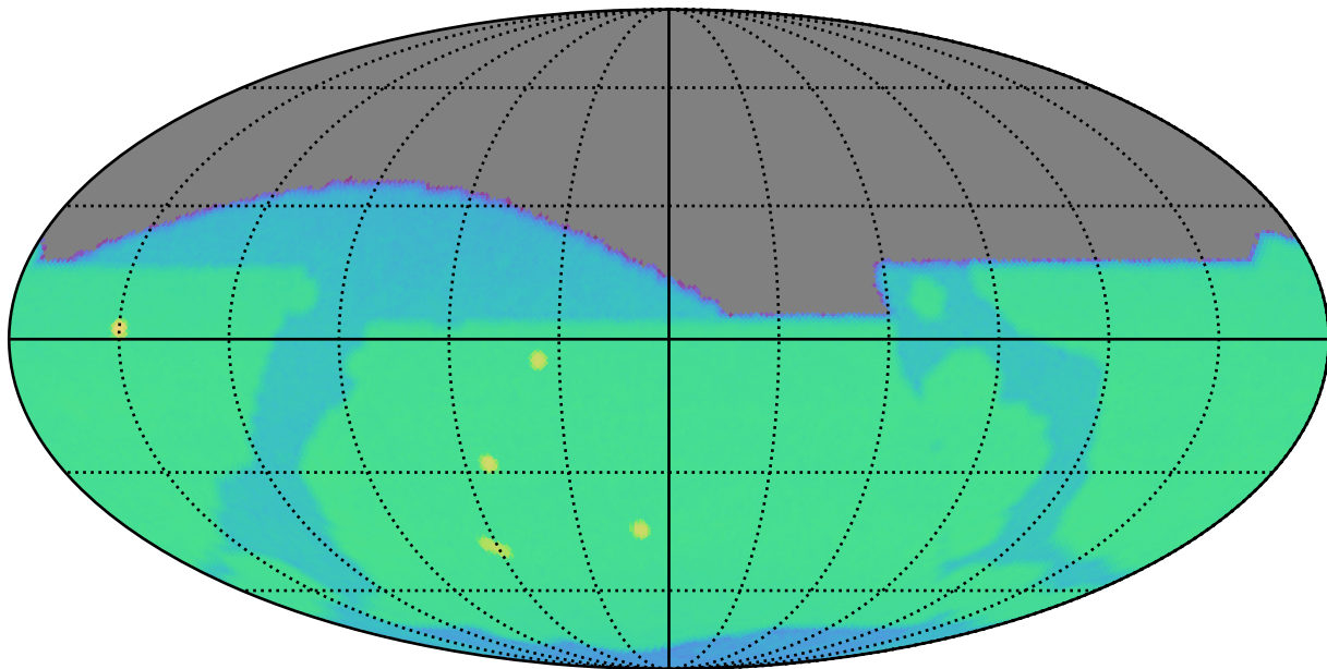
ddf_half_v3.4_10yrs i: SurfaceBrightLimit
