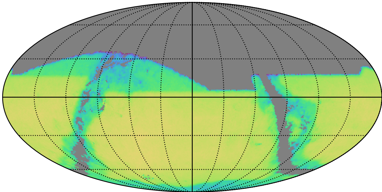
ddf_half_v3.4_10yrs z band and non-DD: QSONumberCountsMetric
