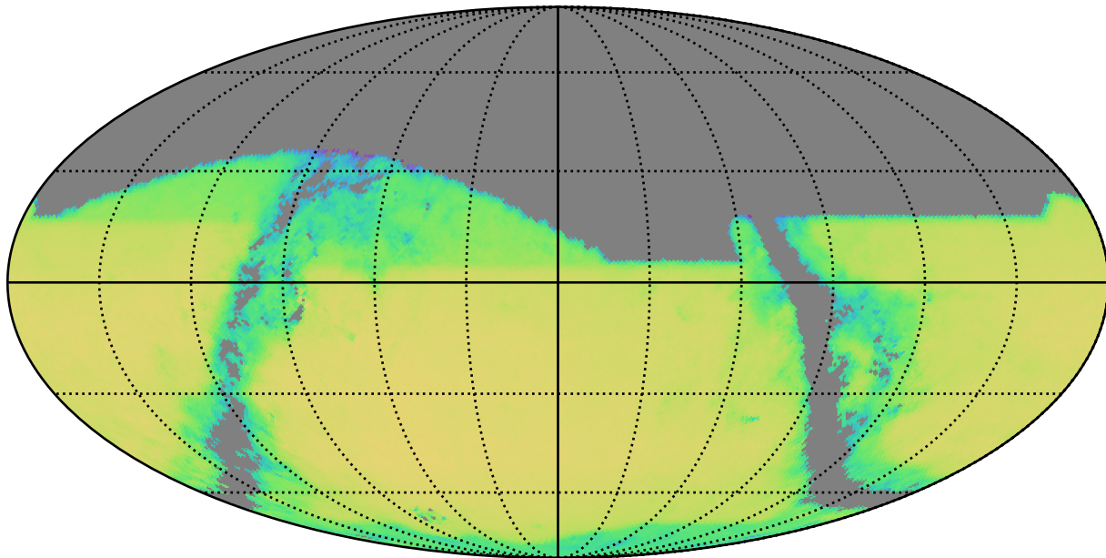
ddf_half_v3.4_10yrs r band and non-DD: QSONumberCountsMetric
