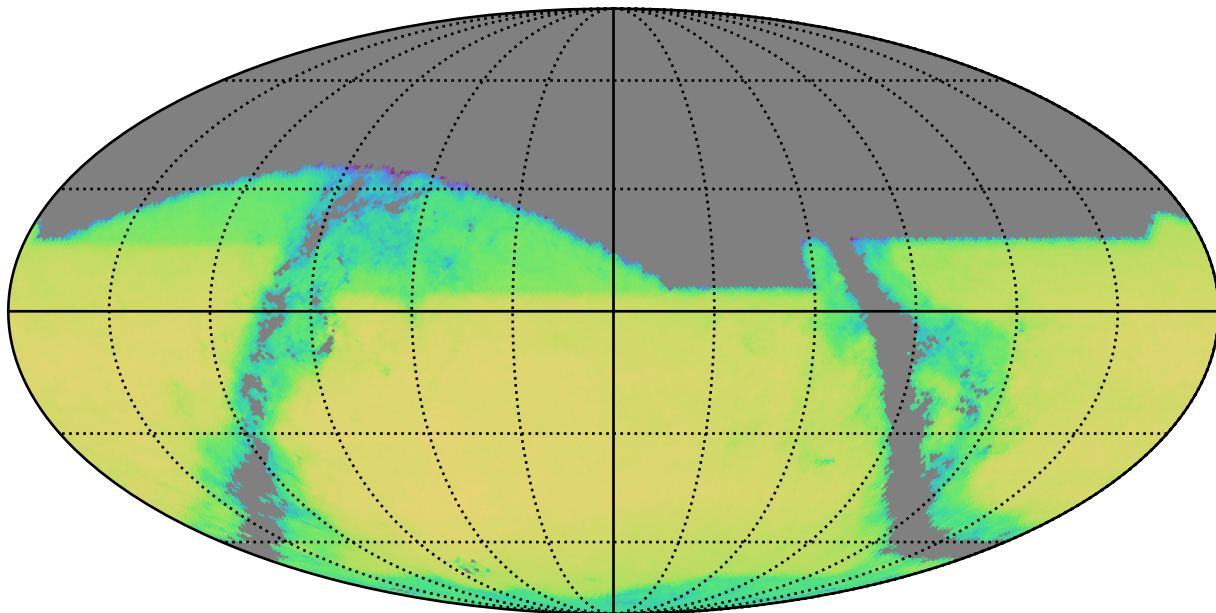
ddf_half_v3.4_10yrs i band and non-DD: QSONumberCountsMetric
