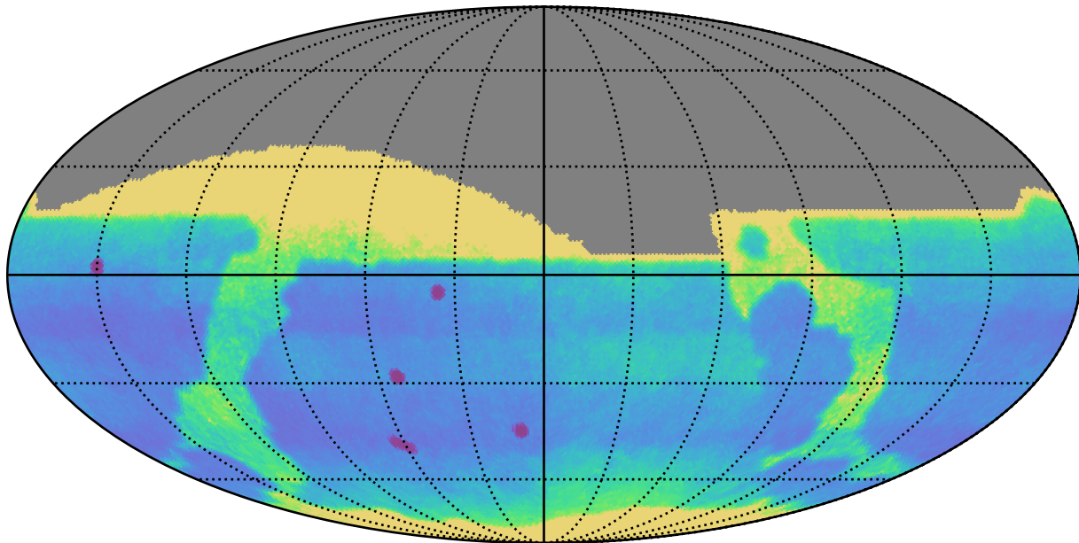
ddf_half_v3.4_10yrs : Proper Motion Uncert @ 24.0
