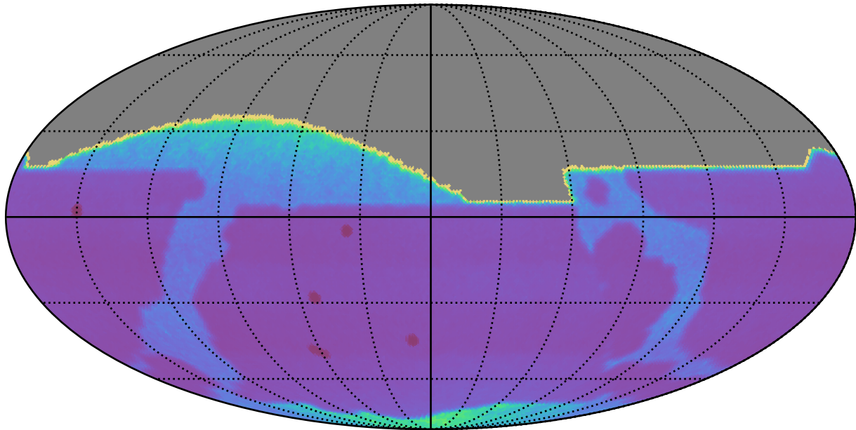
ddf_half_v3.4_10yrs : Proper Motion Uncert @ 20.5
