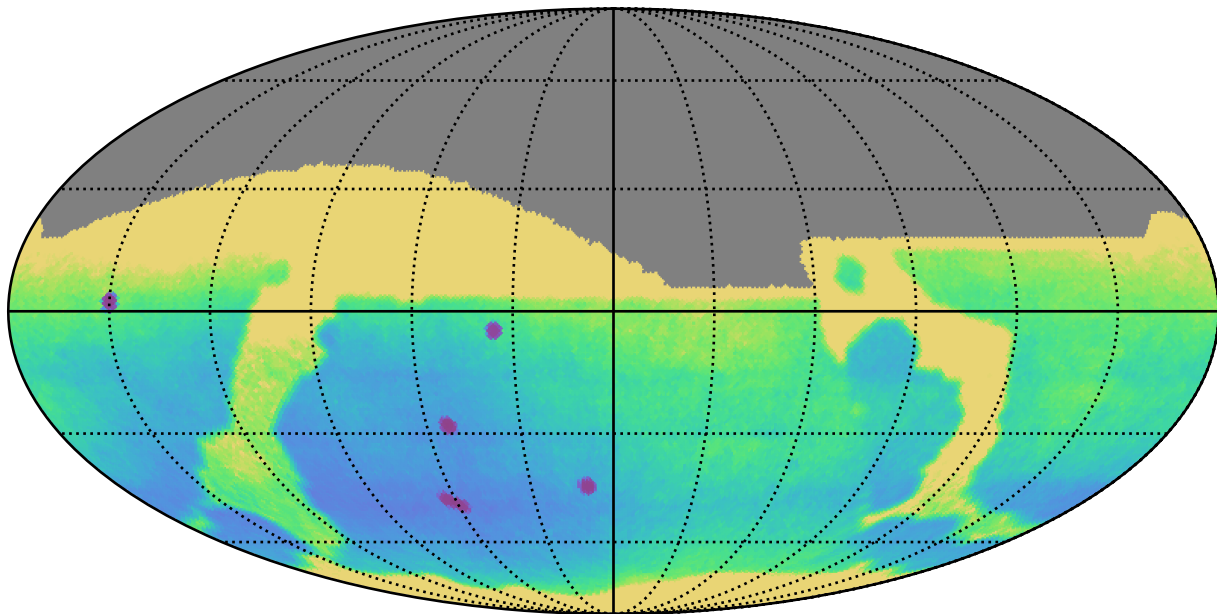
ddf_half_v3.4_10yrs : Parallax Uncert @ 24.0
