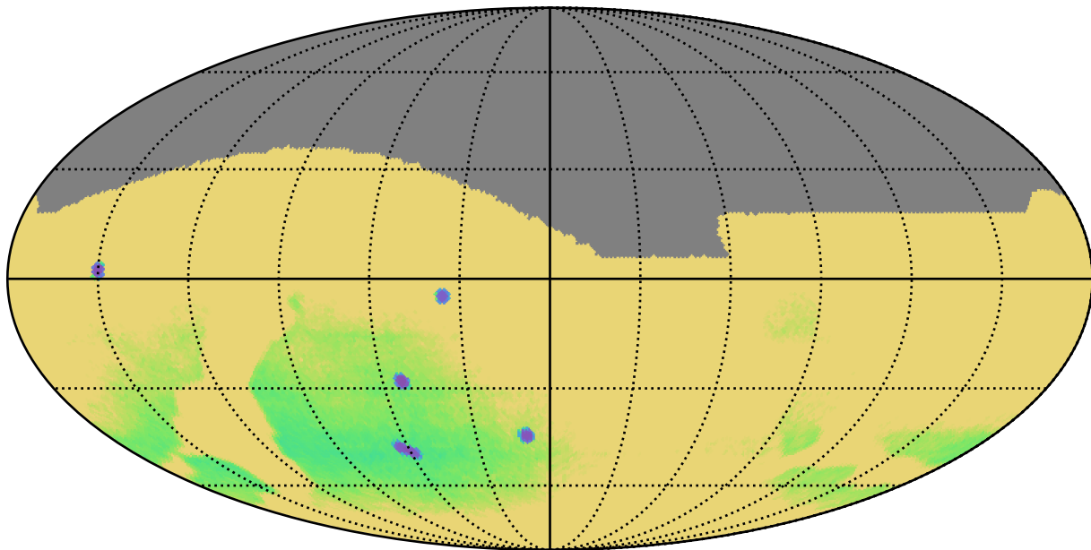
ddf_half_v3.4_10yrs : Parallax Uncert @ 22.4
