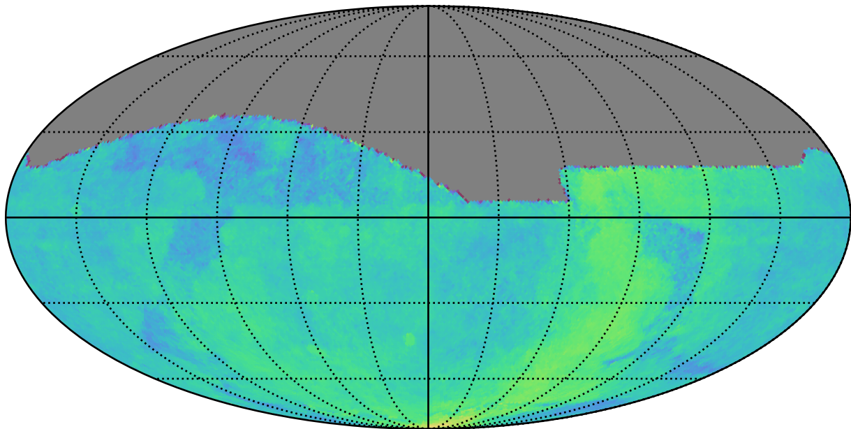
ddf_half_v3.4_10yrs : Parallax Coverage @ 24.0
