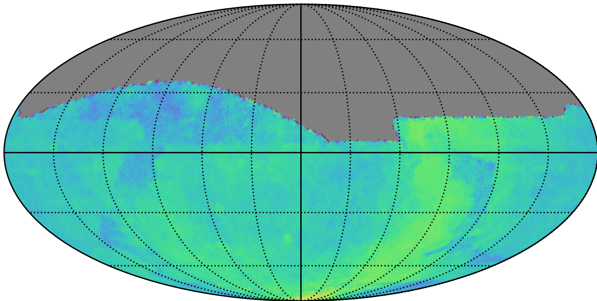
ddf_half_v3.4_10yrs : Parallax Coverage @ 22.4
