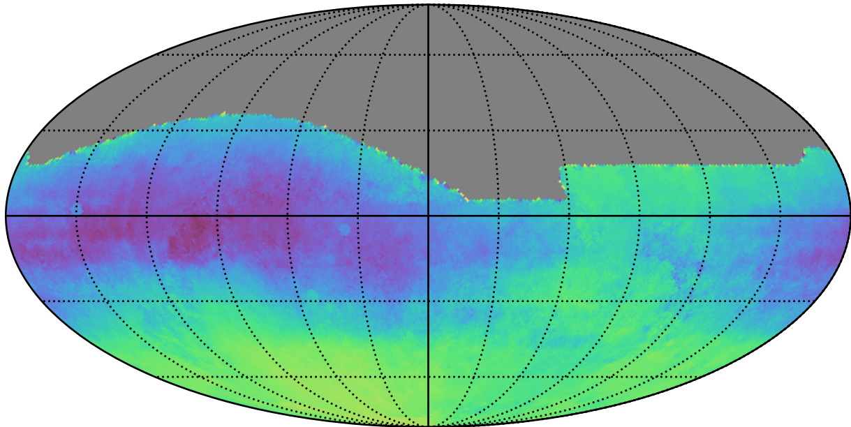
ddf_half_v3.4_10yrs : Parallax-DCR degeneracy @ 24.0
