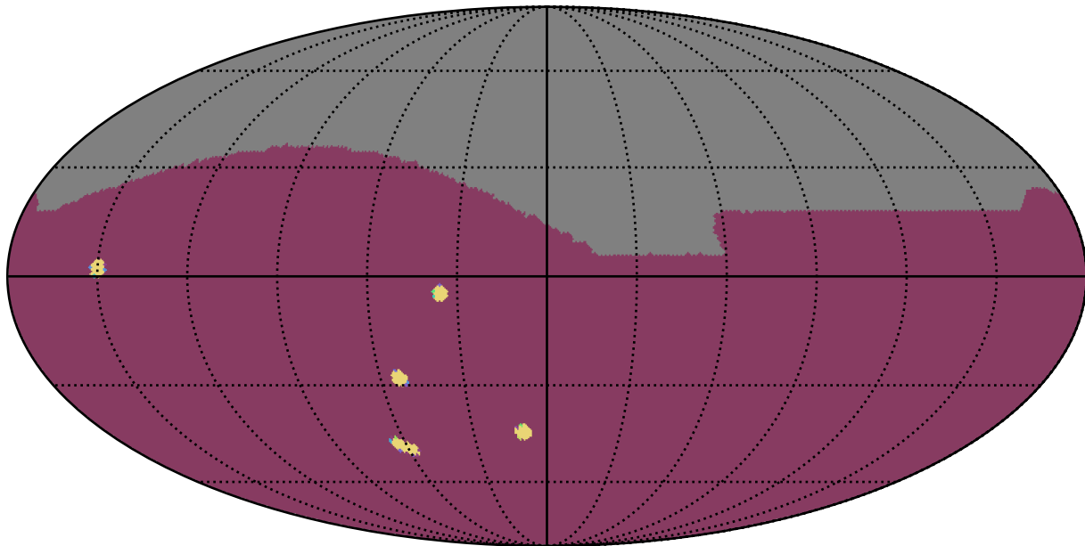
ddf_half_v3.4_10yrs : NumberOfQuickRevisits
