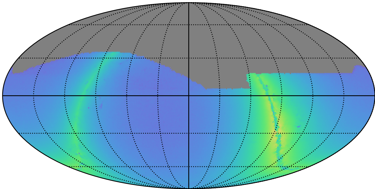
ddf_half_v3.4_10yrs z: Nstars_no_crowding
