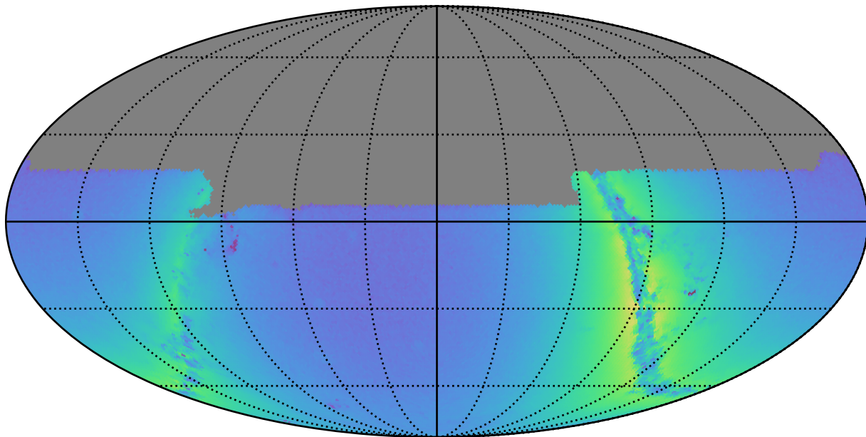
ddf_half_v3.4_10yrs u: Nstars_no_crowding
