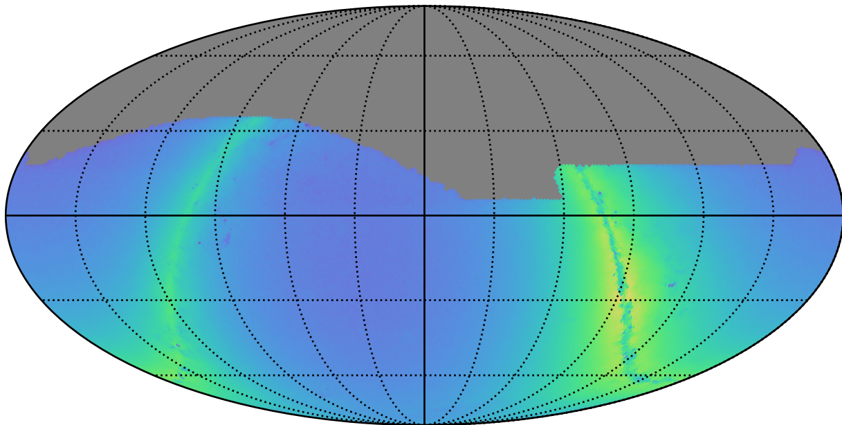
ddf_half_v3.4_10yrs r: Nstars_no_crowding
