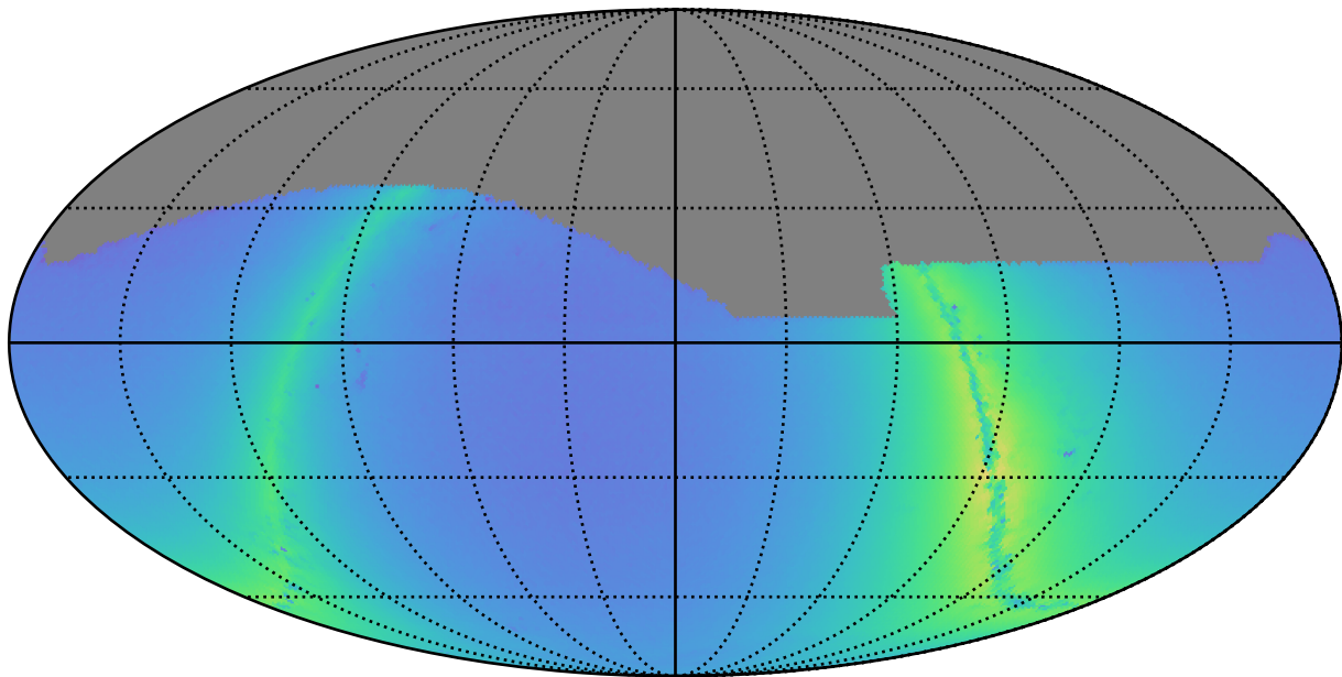
ddf_half_v3.4_10yrs i: Nstars_no_crowding
