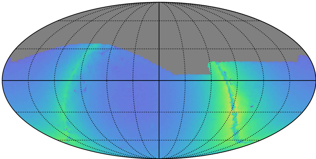
ddf_half_v3.4_10yrs g: Nstars_no_crowding
