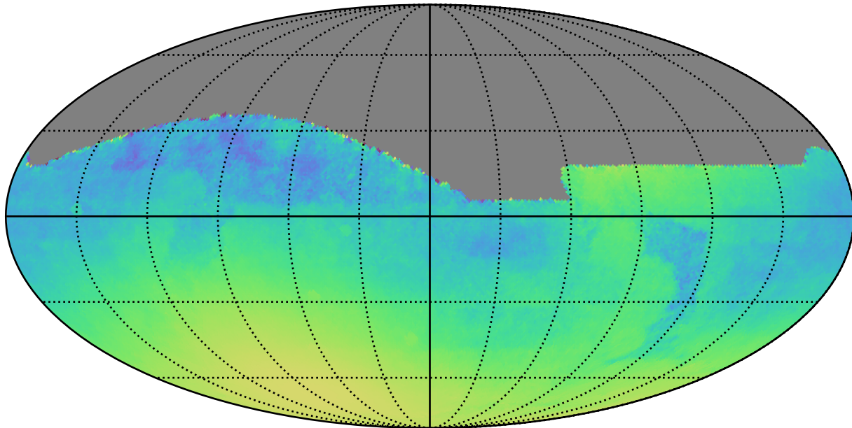
ddf_half_v3.4_10yrs : Normalized Parallax Uncert @ 24.0
