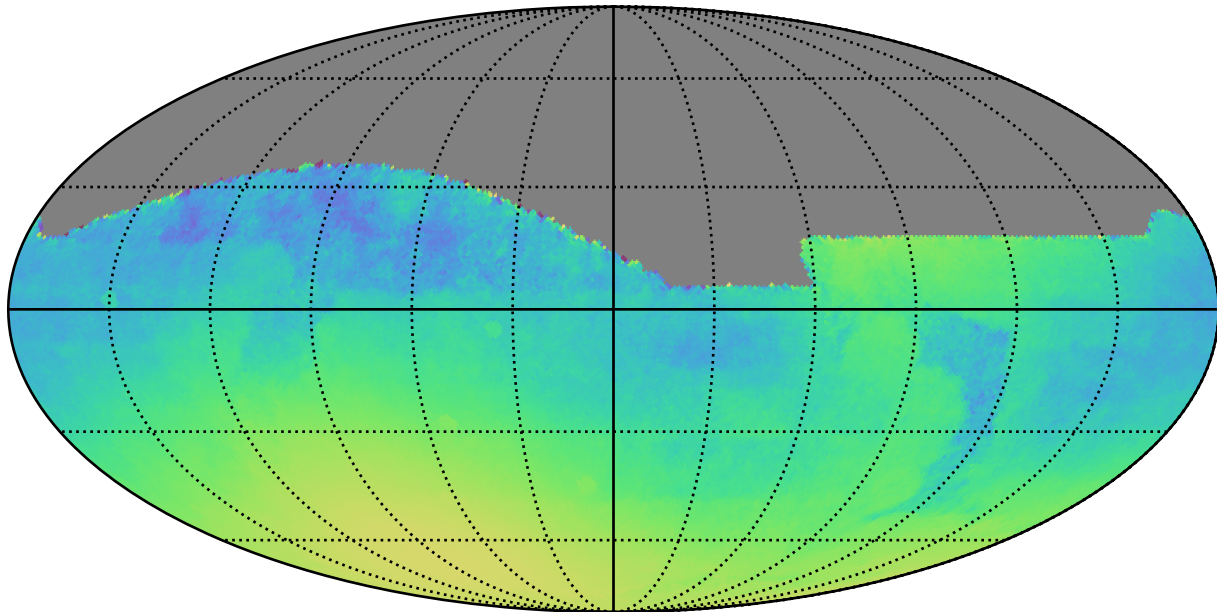
ddf_half_v3.4_10yrs : Normalized Parallax Uncert @ 22.4
