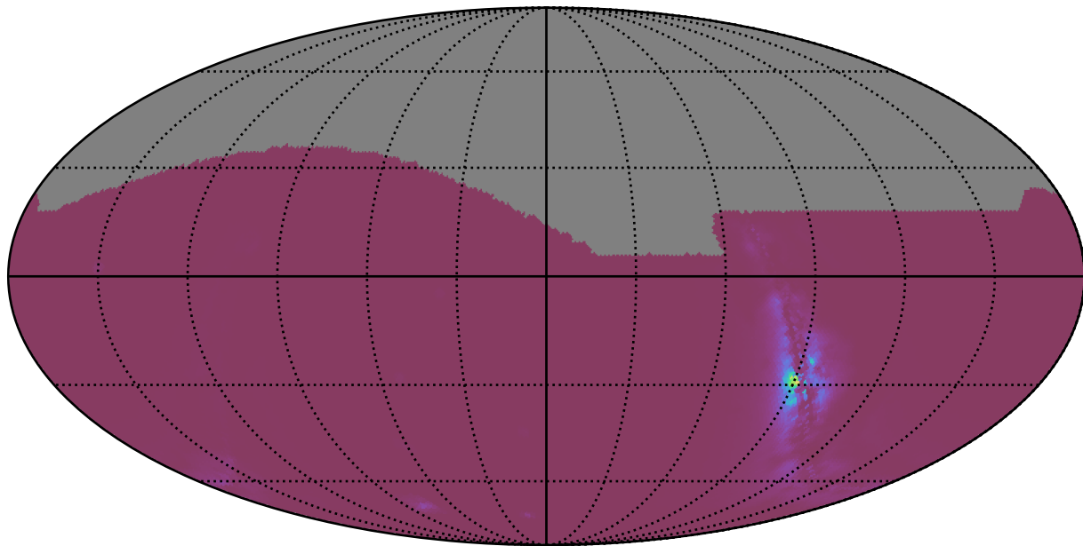
ddf_half_v3.4_10yrs : NlcPoints
