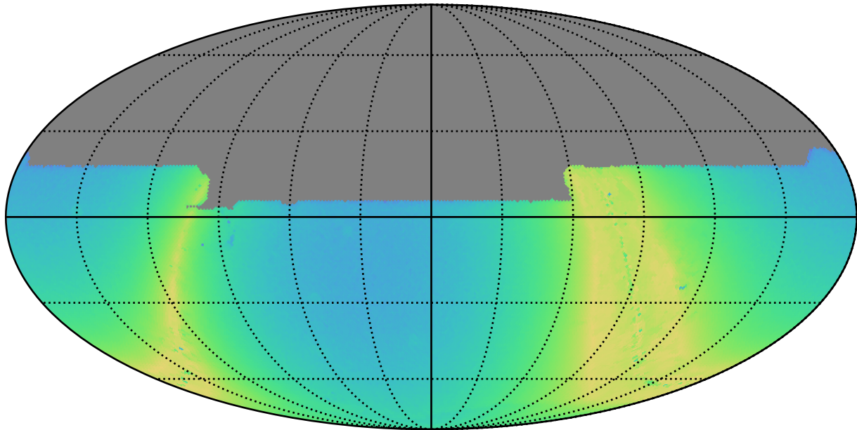
ddf_half_v3.4_10yrs y: N stars to Precision 0.20
