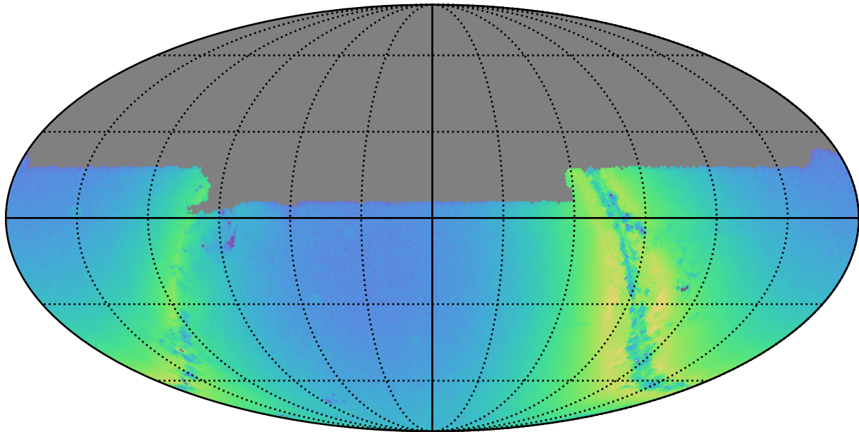
ddf_half_v3.4_10yrs u: N stars to Precision 0.20
