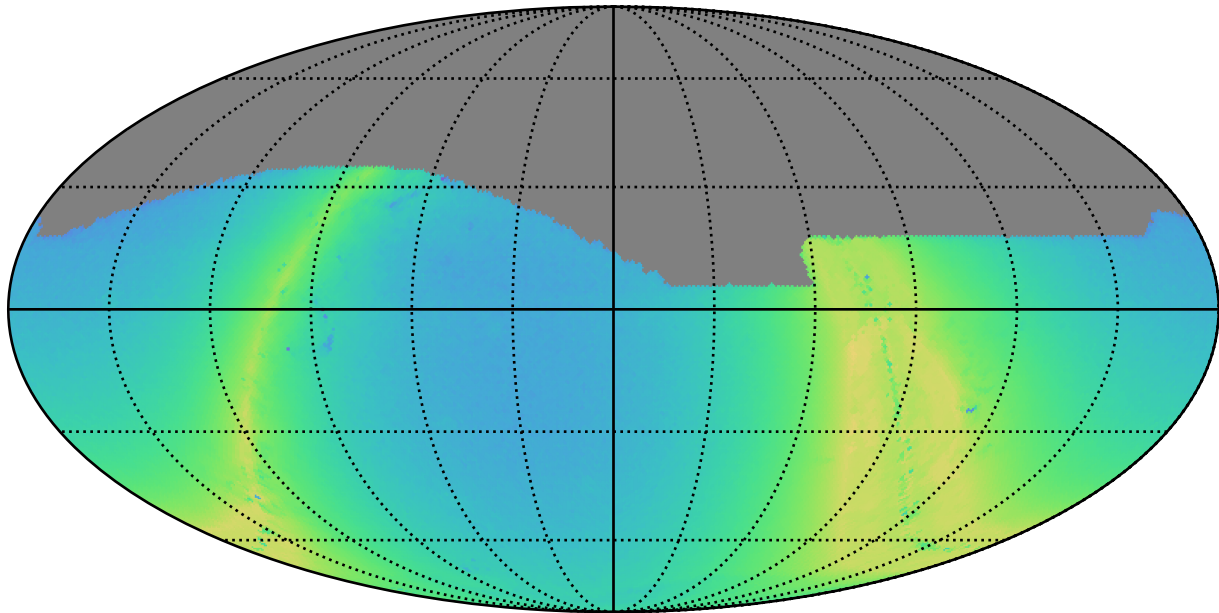
ddf_half_v3.4_10yrs r: N stars to Precision 0.20
