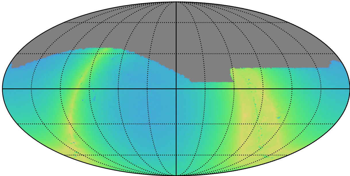
ddf_half_v3.4_10yrs i: N stars to Precision 0.20
