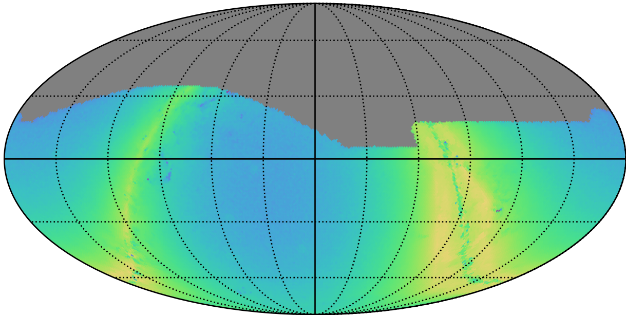
ddf_half_v3.4_10yrs g: N stars to Precision 0.20
