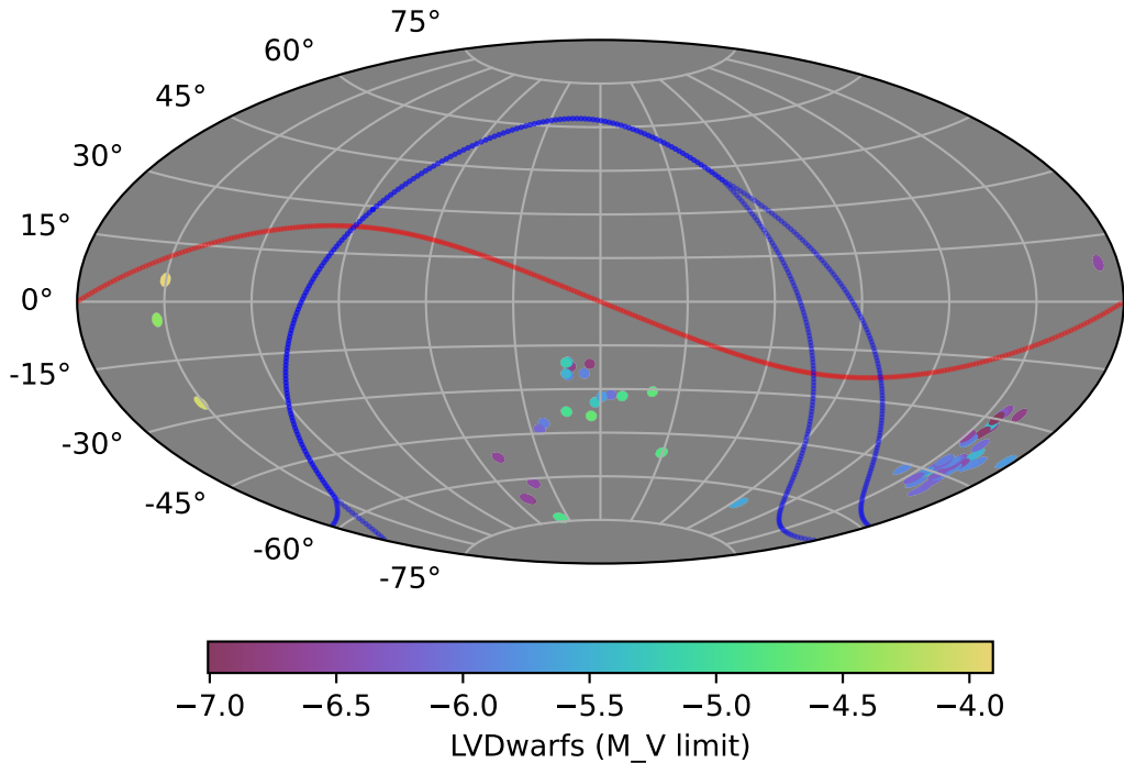
ddf_half_v3.4_10yrs gi: LVDwarfs
