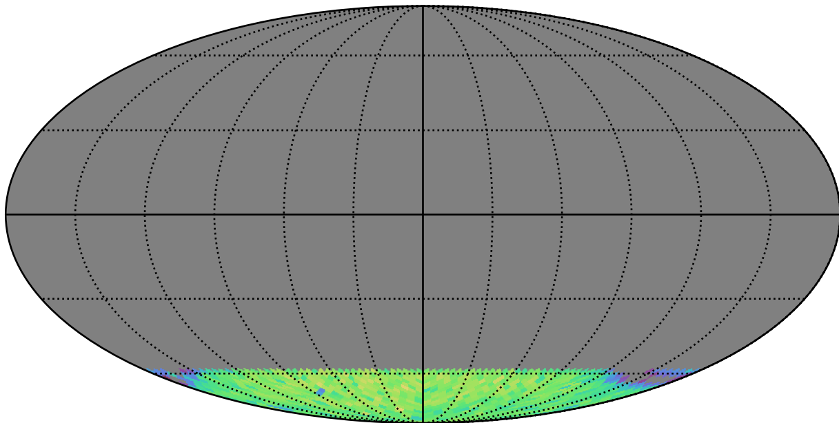
ddf_half_v3.4_10yrs gi SCP: LVDwarfs
