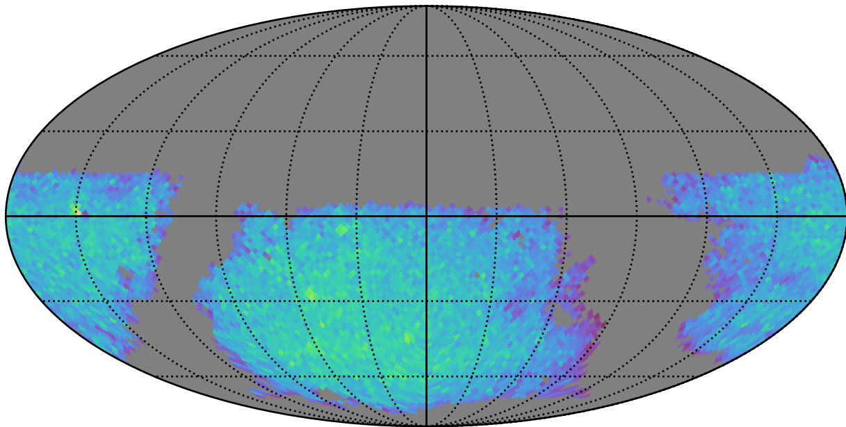
ddf_half_v3.4_10yrs gi: LVDwarfs
