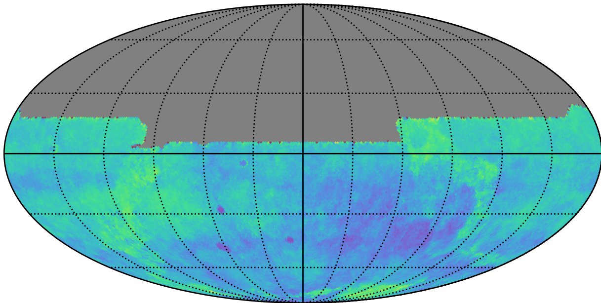
ddf_half_v3.4_10yrs y: Kuiper rotSkyPos
