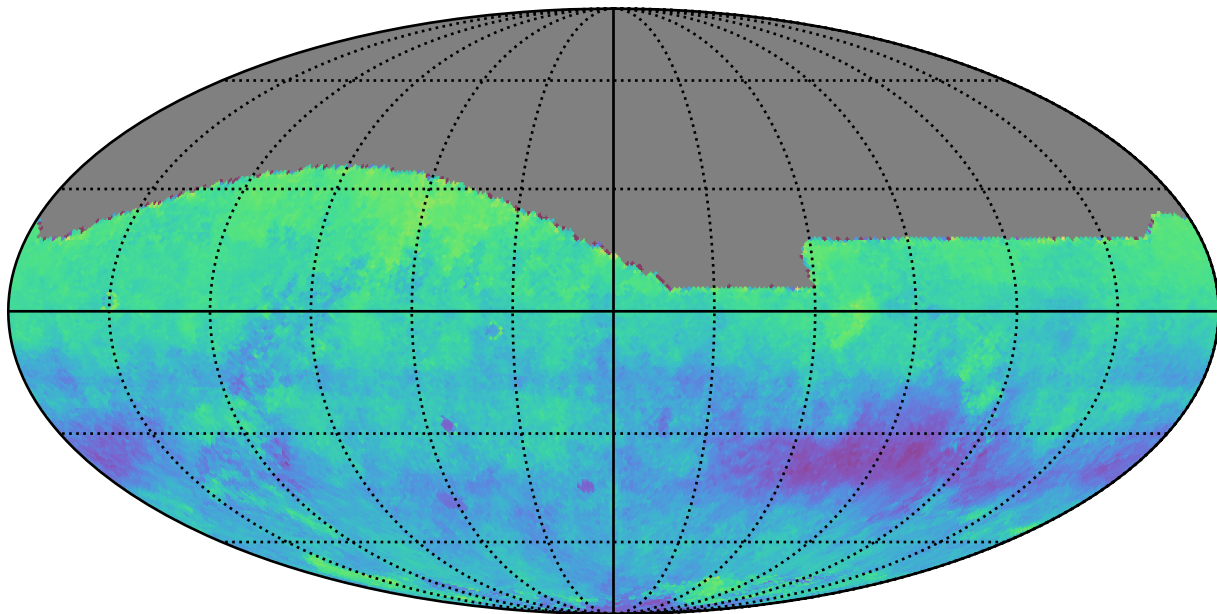
ddf_half_v3.4_10yrs r: Kuiper rotSkyPos
