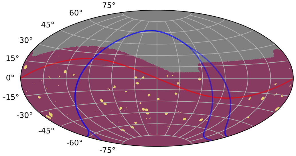
ddf_half_v3.4_10yrs all models: KNePopMetric_all_red_color_detect
