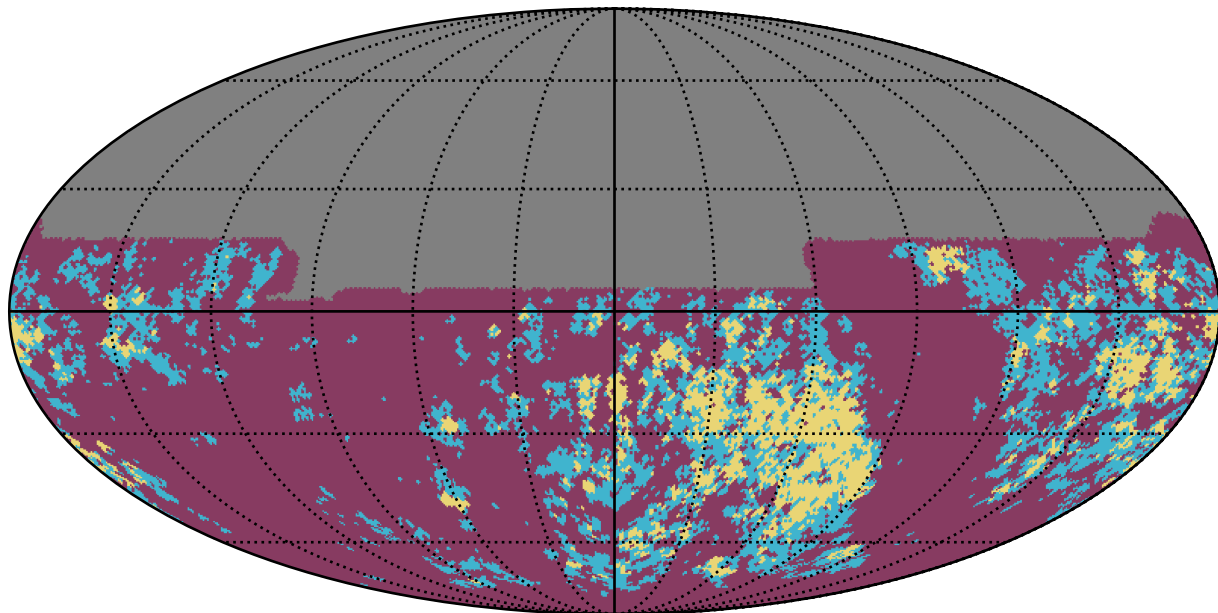
ddf_half_v3.4_10yrs y band: Gaps_7hr
