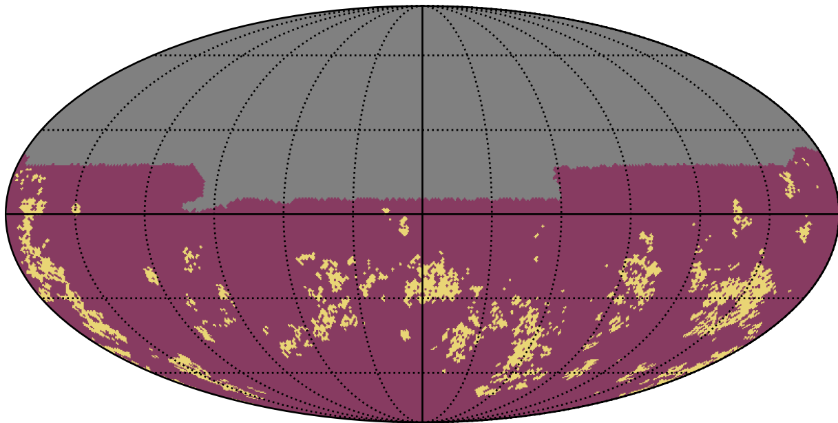
ddf_half_v3.4_10yrs u band: Gaps_7hr
