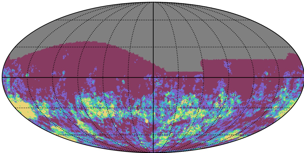
ddf_half_v3.4_10yrs r band: Gaps_7hr
