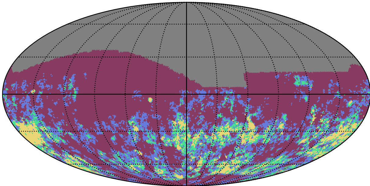
ddf_half_v3.4_10yrs i band: Gaps_7hr
