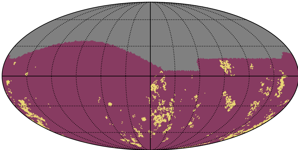
ddf_half_v3.4_10yrs g band: Gaps_7hr
